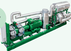
afilia water C-S-r 534 kW th to 2,287 kW th
